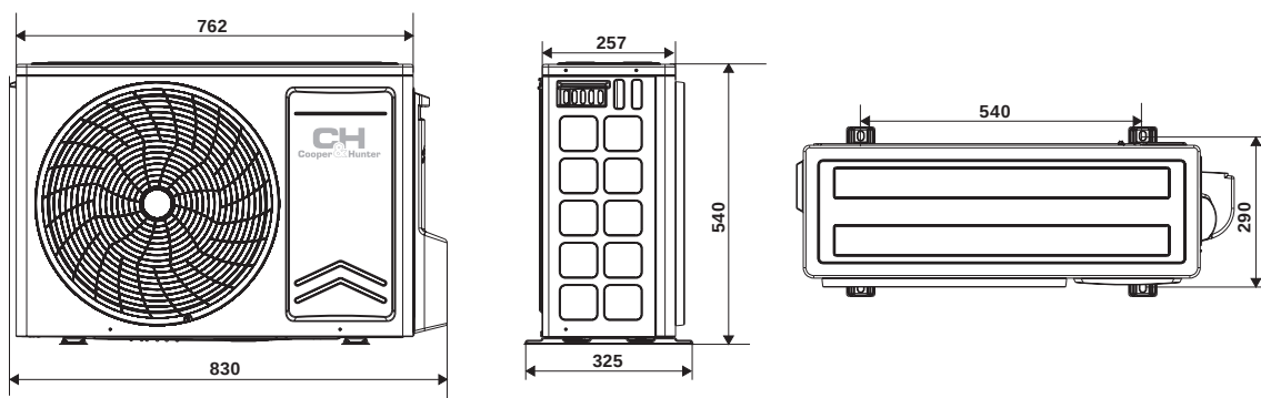
CH-S09FTXN-PS/PW CH-S12FTXN-PS/PW
