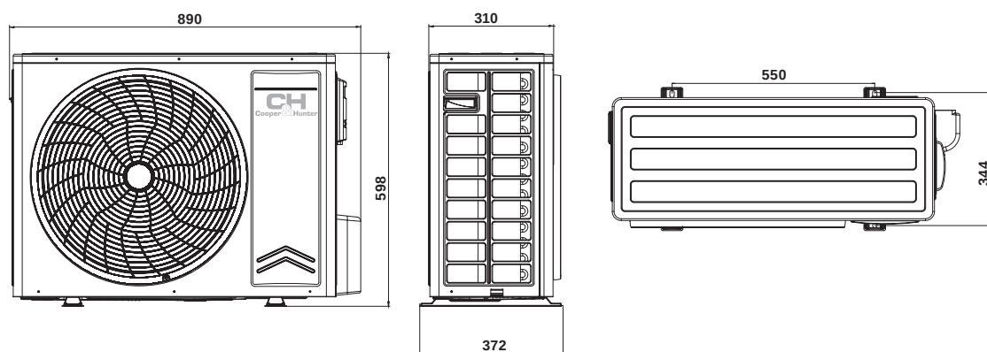
CH-S18FTXN-PS/PW
