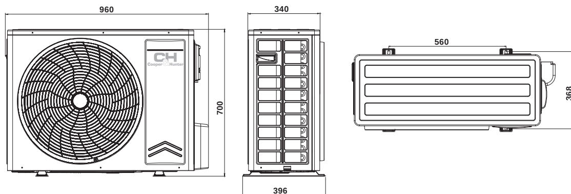
CH-S24FTXN-PS/PW
